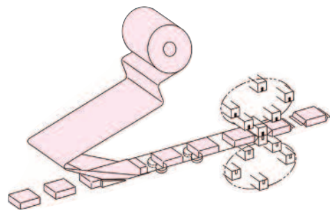
Box-motion type sealer & cutter
