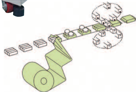
Box-motion type sealer & cutter
