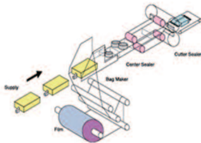
Rotary type sealer & cutter
